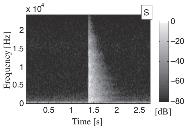
Fig. 7 Spectrogram of impulse response obtained by our proposed method of reducing nonlinear error.
